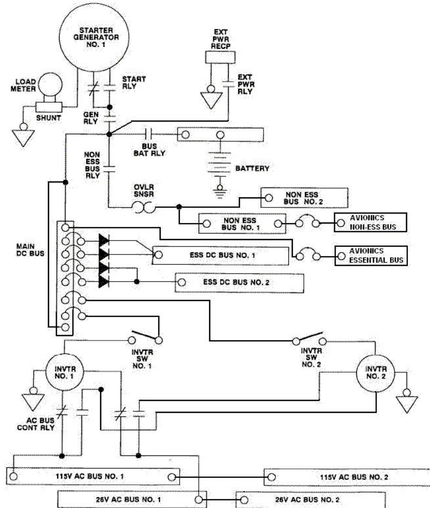
Figure 1-4 – Electrical System Schematic
