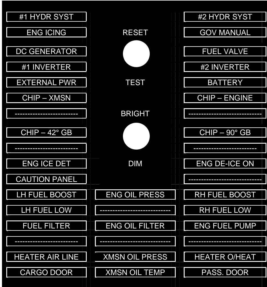
Figure 1-5 – Master Caution/Warning Panel – Typical
