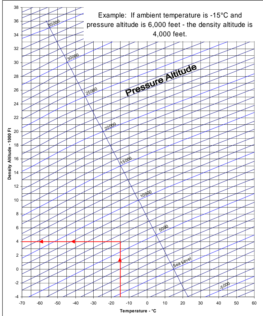
Figure 3-1 – Density Altitude
